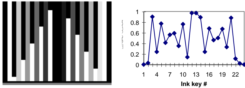
Figure 12. The test plate (left) and plate coverage (right). Zero coverage for Key 1 and 24 was due to the narrower web width.
