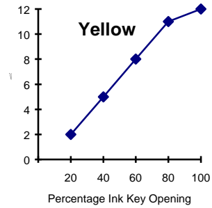
Figure 10. Relationship between ink key opening and ink film thickness on ink fountain rollers.
