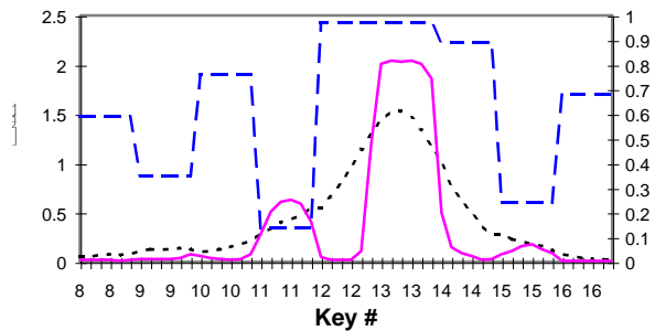
Figure 8. Ink distribution with vibrators on (dotted curve) and off (solid curve). The dashed curve is zonal coverage.
