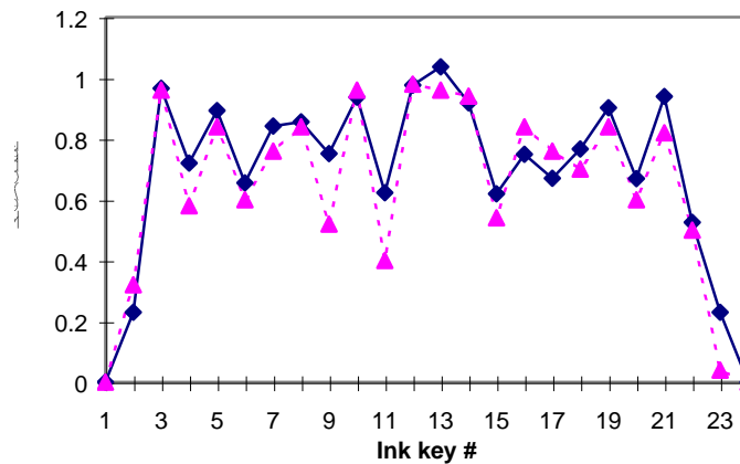
Figure 13. Ink key presetting: model (diamonds) vs. actual (triangles).
